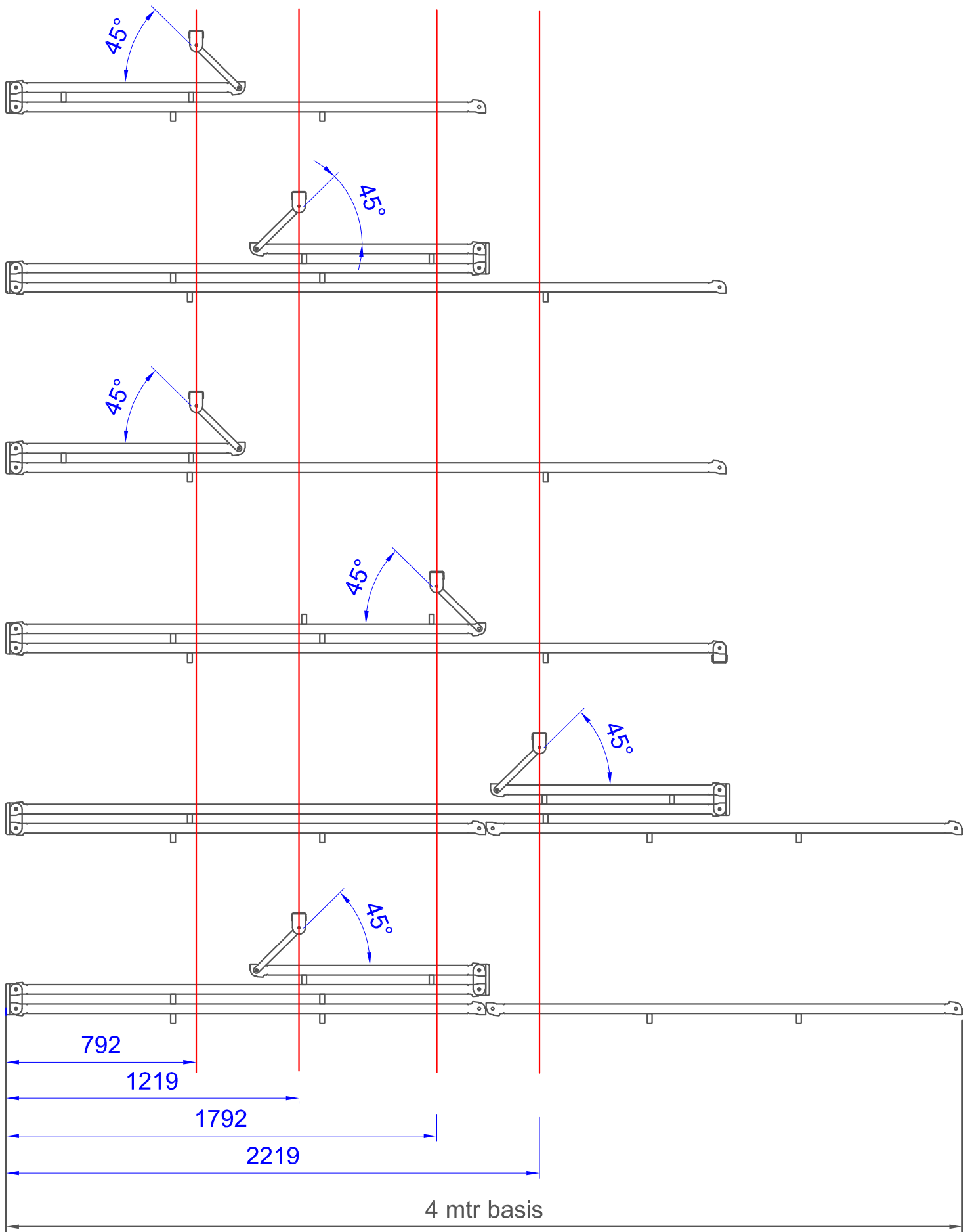
foundation measurements
