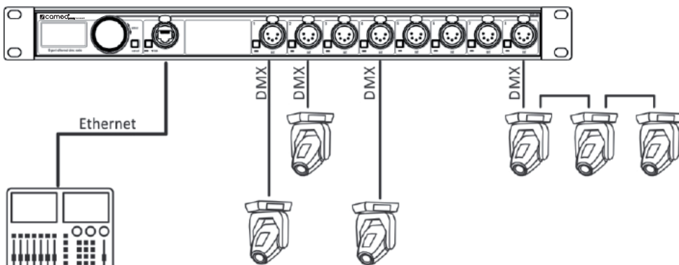
Lighting Controller
