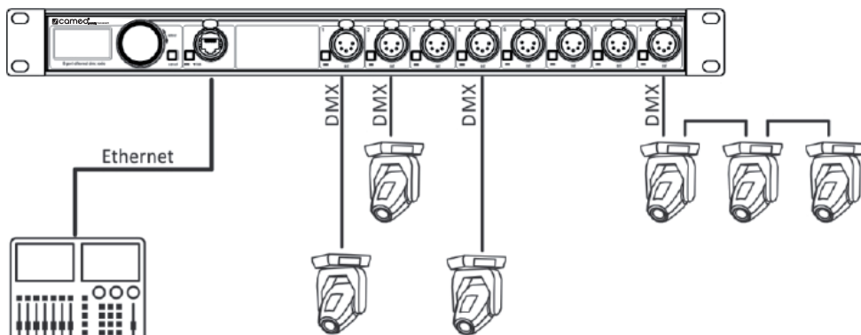
Lighting Controller
