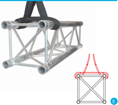
RECTANGULAR TRUSS | 1 SLING WRAP UPPER CHORDS
