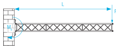
Catilvear lengths L, Force F, Bending moment M_b Formula M_b = F \times L
