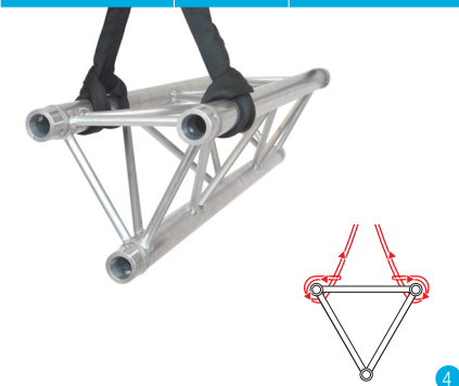
TRIANGULAR TRUSS APEX DOWN 2 SLINGS CHOKED
