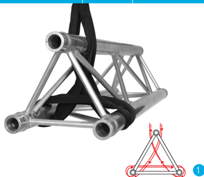
TRIANGULAR TRUSS APEX UP 1 SLING BASKET
