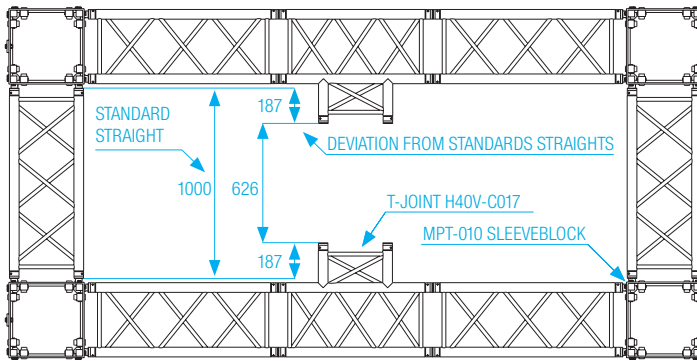
Figure: H40V-C017 with MPT seeve blocks
