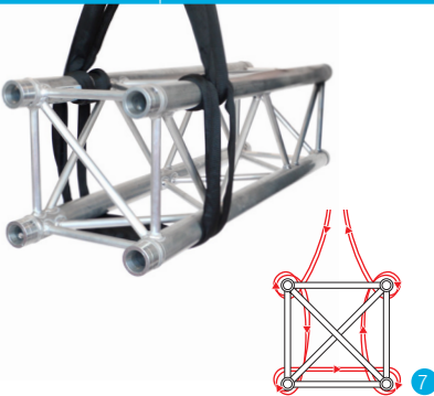
RECTANGULAR TRUSS | 2 SLING CHOKE UPPER CHORDS
