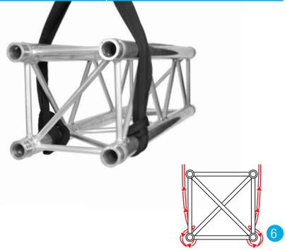
RECTANGULAR TRUSS | 2 SLING CHOKE LOWER CHORDS
