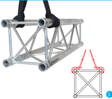
RECTANGULAR TRUSS | 2 SLING CHOKE UPPER CHORDS
