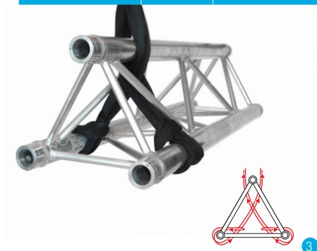
TRIANGULAR TRUSS APEX UP 2 SLINGS CHOKED
