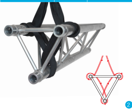
TRIANGULAR TRUSS APEX DOWN 1 SLING WRAP
